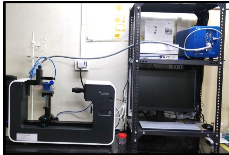
Insitu wettability-electrochemical behavior evaluation setup
