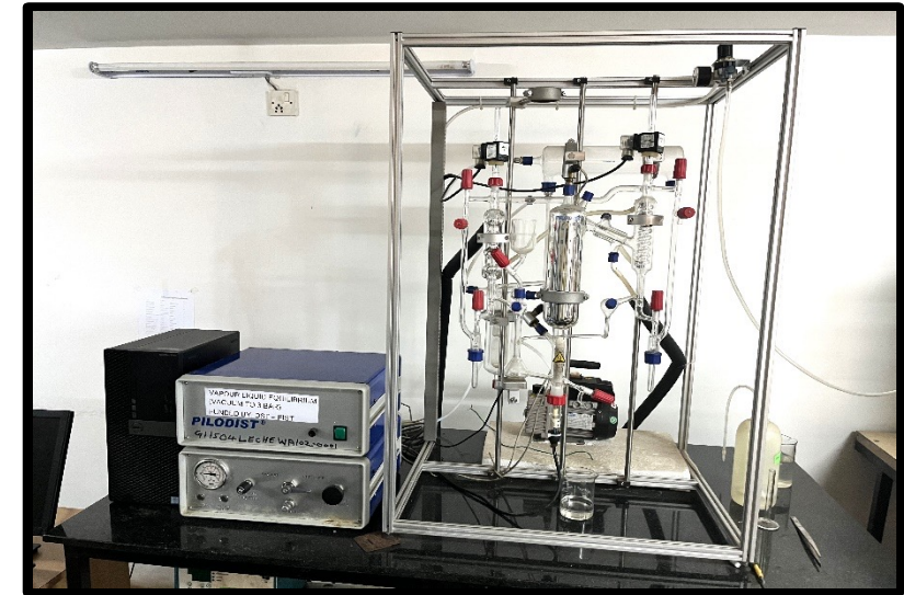
VLE SETUP
