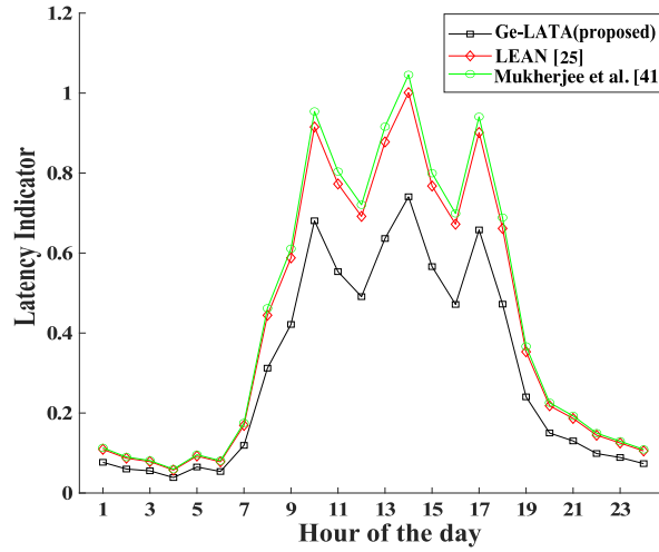
Fig. 4. Latency variation during a sunny day.
