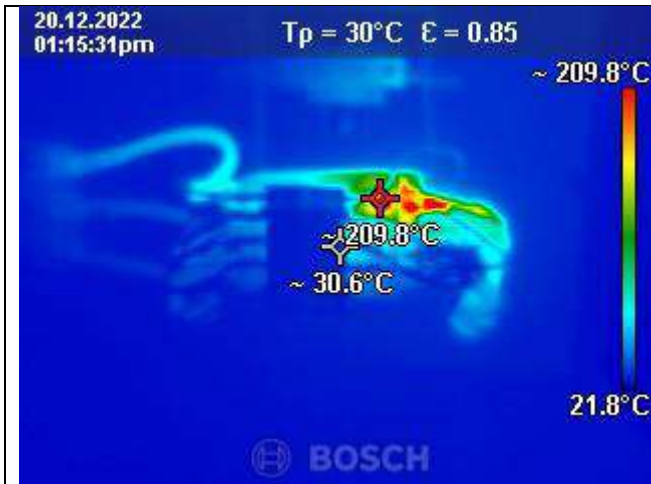
Location – Transformer 2 Capacitor bank 13F3 50 kVAR
