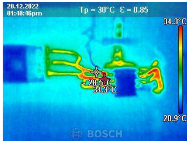
Location – Transformer 3 Capacitor bank 7F3 25 kVAR
